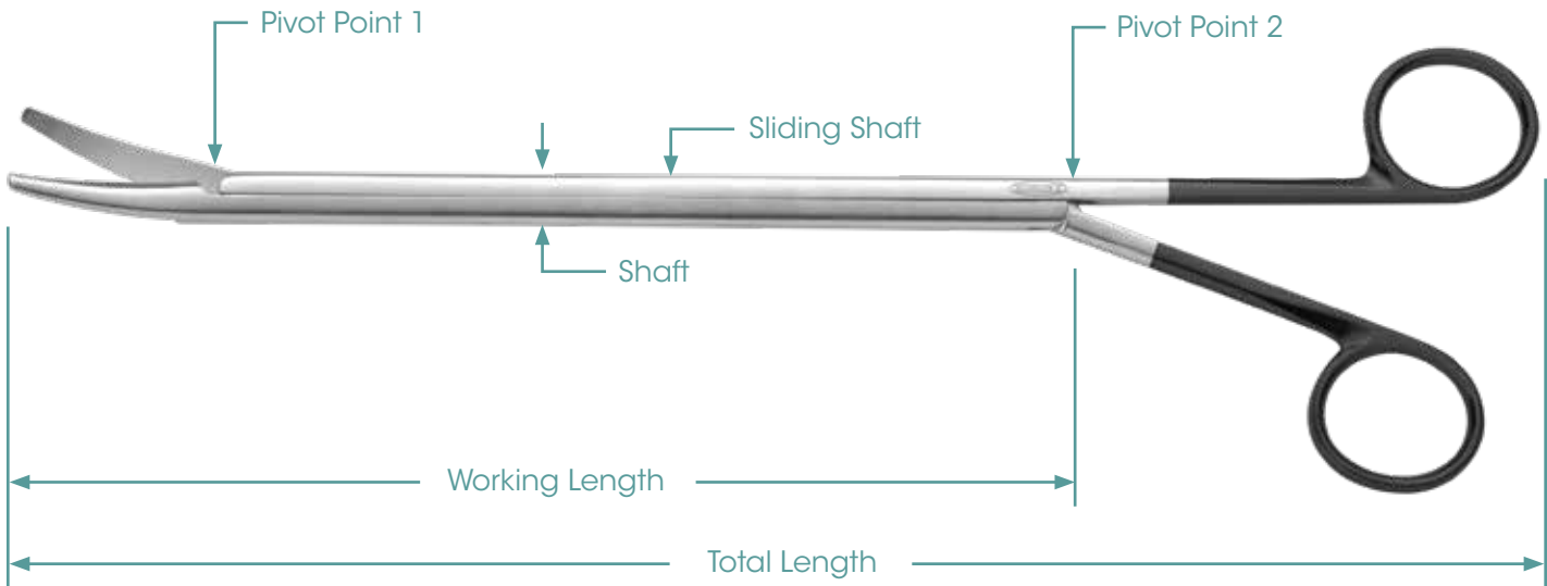
VATS Scissors 9909-910SC
